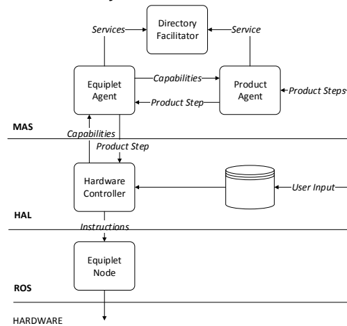
Figure 6: System dependencies
