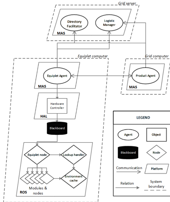
Figure 3: Software Architecture
